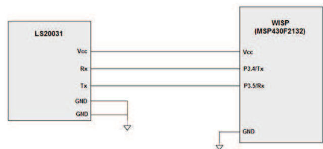
Fig. 4. Block Diagram of GPS receiver and WISP interfacing
