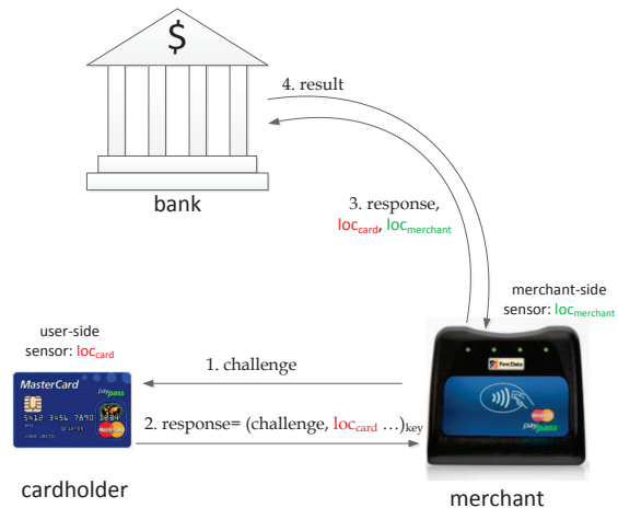
Fig. 3. Online authorization in a mobile payment system enhanced with our proximity detection approach
