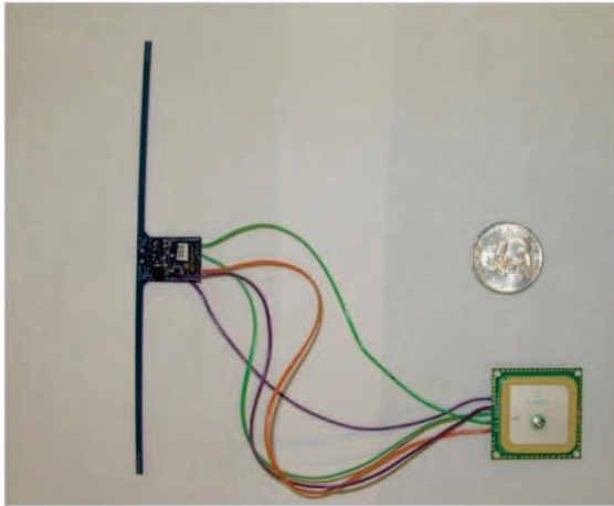
Fig. 5. GPS interfaced with the WISP
