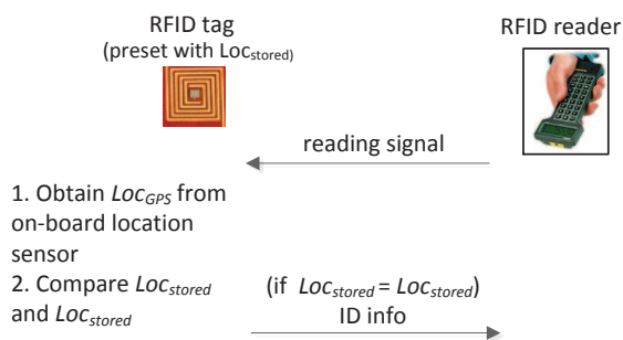
Fig. 2. Location-aware selective unlocking where Loc_{stored} is legitimate location (or speed) info stored on the tag side and Loc_{GPS} is the location info obtained from on-board GPS upon a reader request.
