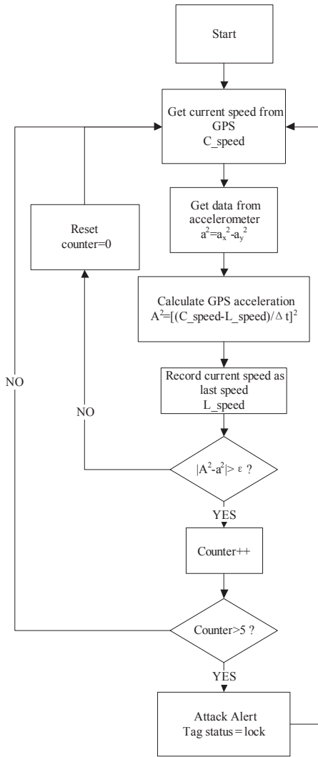
Fig. 6. Flow chart for detecting GPS spoofing attack
